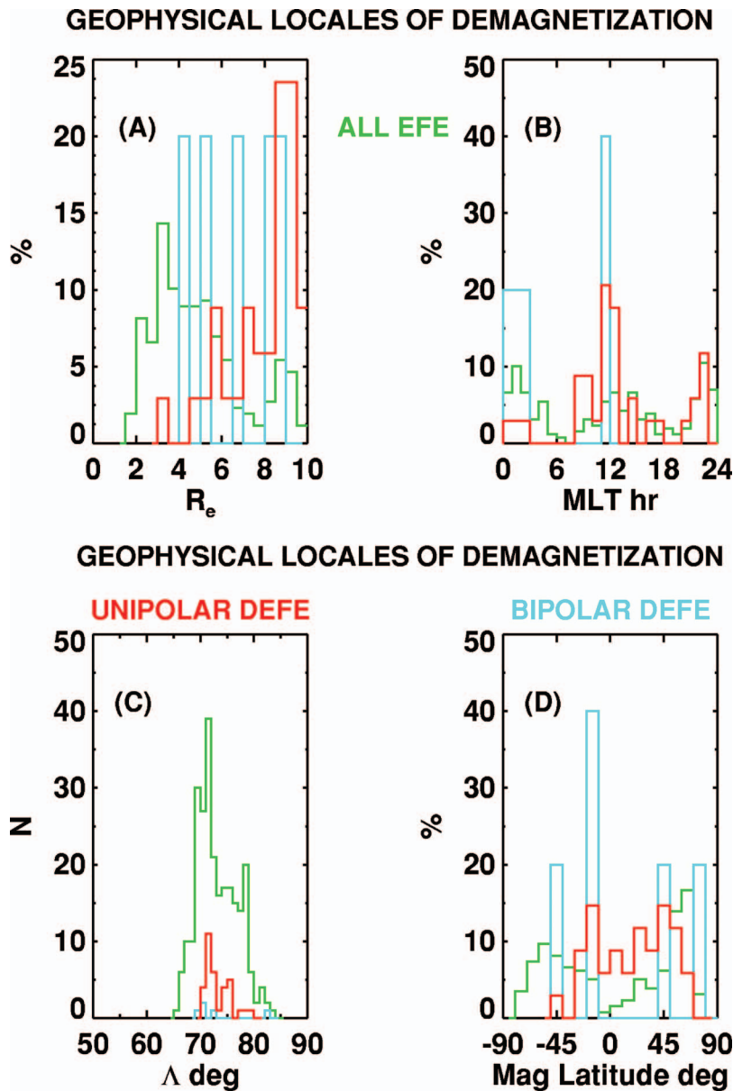
FIG. 11. (Color). Geophysical locales of EFES: (a) radius in Earth radii; (b) MLT hours (noon=12); (c) invariant magnetic latitude, \Lambda (degrees); (d) magnetic latitude, (degrees). All EFES in green; unipolar DEFES (red); and bipolar DEFES (cyan-aqua).
