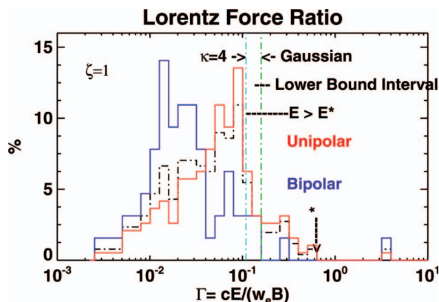
FIG. 8. (Color). Observed distribution of Lorentz force ratio, \Gamma_{obs} = cE_{obs}/(w_{e,obs}B_{obs}) . Black histogram: all EFE; red: unipolar EFE; blue: bipolar EFE. Vertical dashed green and cyan lines are theoretical values for \Gamma_{theory}(a=1) determined from Gaussian or kappa velocity distribution averages reflected in Eqs. (15) and (16), respectively. The asterisk denotes the location of the only EFE event (Ref. 8), whose spatial scales are known by measurement; it is clearly shown here as a DEFES.
