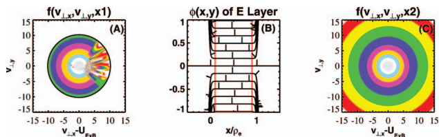
FIG. 4. (Color). Summary of detailed integrations of equation of motion for electrons (through an EFE as illustrated in inset B) connecting points of observation at two points (A) and (C) well removed from any gradients in \mathbf{E} . Use has been made of Liouville's theorem. Isocontours are made of velocity space in the equatorial plane with the magnetic field as its pole. Since \mathbf{E} \cdot \hat{\mathbf{B}} = 0 phase space is four-dimensional and all coordinates are resolved here. Velocity distribution at (c) is a generalized Lorentzian, kappa function with \kappa=4 , that is gyrotropic—hence the concentric phase space zones. Since the Hamiltonian is time independent the trajectories are time reversible, and the phase space at (a) is constructed by numerically integrating the equations of motion from (a) to the locale of (c) and “painting” the distribution function in (a) accordingly. \Gamma=0.1 at threshold has been assumed. Mapping done at 5^\circ increments \Gamma within the black circular border of inset (a). Portions of phase space that are white inside the black circular ring in (a) are locales where connection trajectories could not be found. These regions invariably adjoin phase space regimes reflecting nongyrotropic access. No phase space matching was attempted outside the black circular border in inset (a) since the trajectories required too much computer time. Note distortions in that part of velocity space that determine the maximum contribution to the pressure tensor elements.
