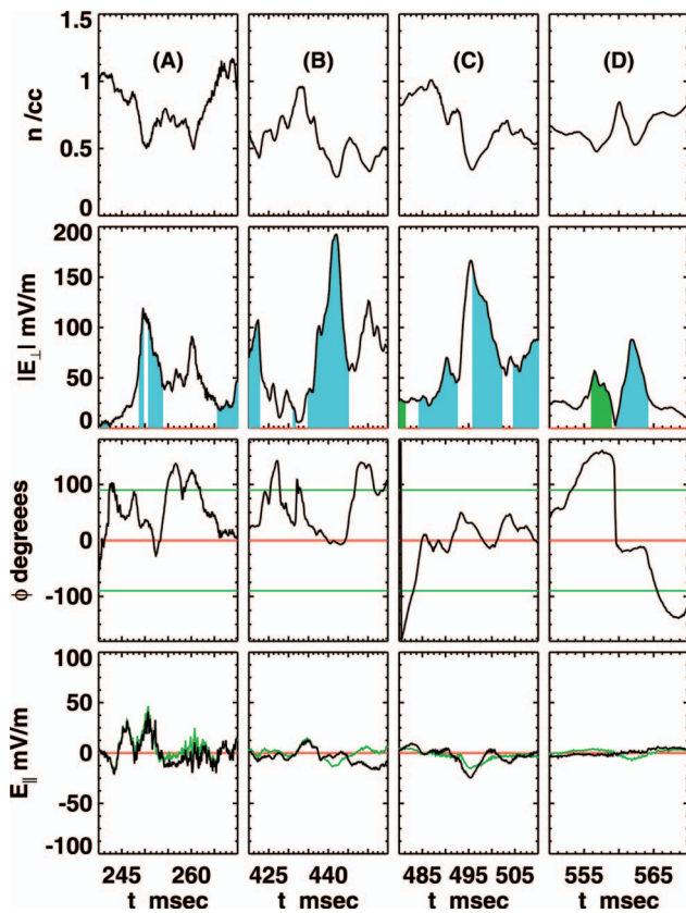
FIG. 2. (Color). Four insets from Fig. 1 (keyed by corresponding letters), showing the laminar character of the resolved time series and the correlation of the variations of E_{\perp} with cylindrical phase, and local density variations. Same format as Fig. 1.
