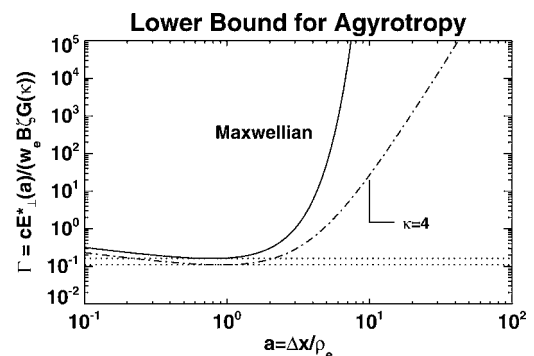
FIG. 6. Theoretical variation of \Gamma(a) = cE_{\perp}^*(a)/(w_e B \zeta G(\kappa)) that determines the lower limit threshold electric field E_{\perp}^*(a) . The function G(\kappa) = (2\kappa/(2\kappa-3))^{1/2} . Since this ratio \Gamma is determined by \mathcal{J}(a)^{-1} , it has a broad minimum in the vicinity of a \approx 1 , while retaining a strong sensitivity to the energy dependence of the phase space distribution of electrons when a > 2 . The minimum threshold for \kappa=4 occurs at \Gamma(a=0.93, \kappa=4) = 0.11 , while that for the Maxwellian distribution occurs at \Gamma(a=0.75, \kappa=\infty) = 0.16 . These two values of \Gamma set the horizontal dashed lines in this figure and set the locations of the cyan and green lines in Figs. 7 and 8.
