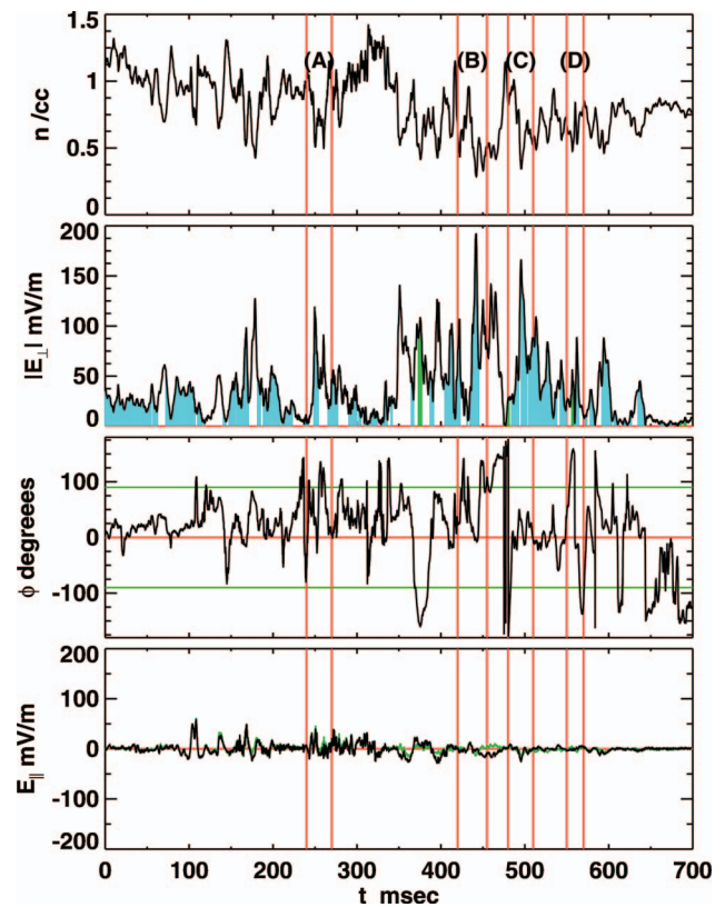
FIG. 1. (Color). Example of an EFE using data capture over 700 ms acquired on NASA's Polar spacecraft on April 1, 2001, starting at 23:24:56.40164UT. “Burst” of high resolution electric field data collected at 800 Hz. From the top, inferred density from probe potentials, magnitude of components of \mathbf{E} perpendicular to \mathbf{B} , phase angle of \mathbf{E}_\perp relative to the direction of minimum variance of \mathbf{E}_\perp , followed by \mathbf{E} \cdot \hat{\mathbf{B}} inferred by two different methods described in the text. Aqua shading indicates locales where the phase of \mathbf{E}_\perp goes through zero. Frequently this is also a peak in \mathbf{E}_\perp . E_\parallel trace is constructed two different ways: green and black trace described in text. Both methods agree that routinely and at the peaks of \mathbf{E}_\perp , that E_\parallel \ll E_\perp .
