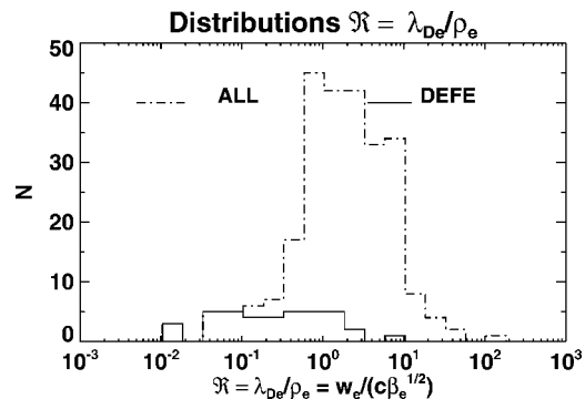
FIG. 10. \mathfrak{X} = \lambda_{De}/\rho_e distribution for DEFES (solid) and all EFES (dashed).
