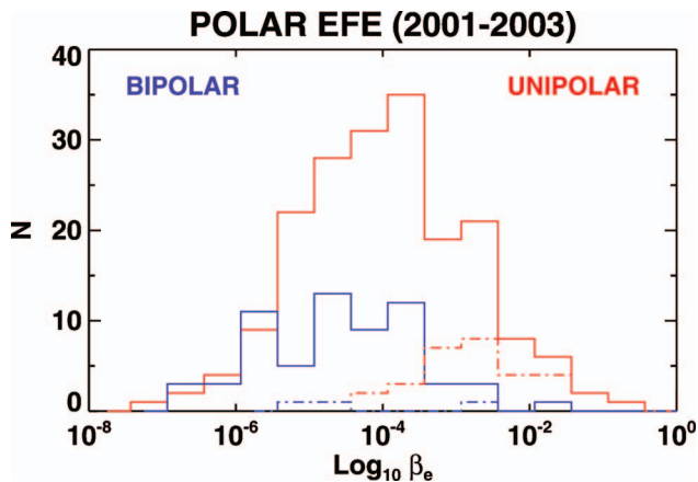
FIG. 9. (Color). \beta_e distribution given by solid histograms for unipolar EFES (red) and bipolar EFES (blue). Corresponding classes of DEFES given by dashed histograms with the same colors. EFES are a very low \beta_e phenomena.
