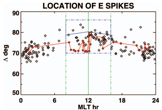
FIG. 12. (Color). MLT- \Lambda distribution: all EFES in black; unipolar DEFES red symbols connected by line segment. Blue dashed box is the recently resurveyed (Ref. 19) boundary of the Earth's, magnetic cusp in the Northern Hemisphere. Vertical green dashed lines indicate \pm 4 h of local noon where DEFES are preferentially found. Next highest local is local midnight.
