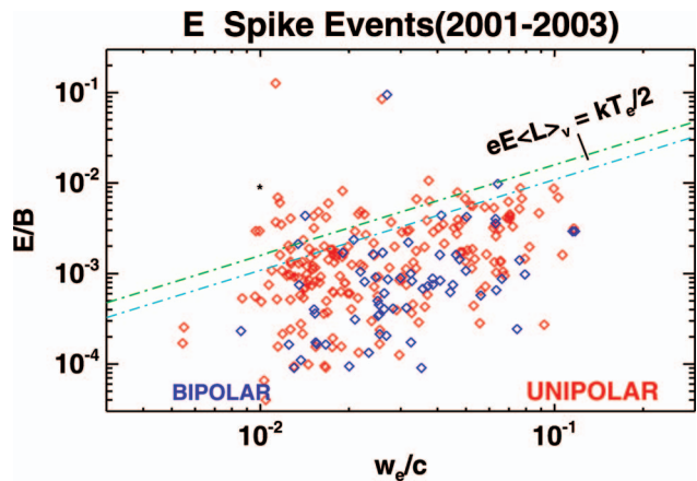
FIG. 7. (Color). E/B vs w_e/c using only observables. Cyan and green dashed lines are theoretical boundaries implied by (15) and (16). The black asterisk is location in parameter space of only EFE event whose spatial scales have been measured (Ref. 8).
