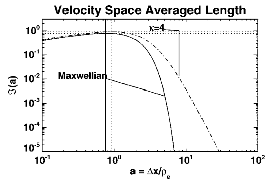
FIG. 5. Velocity spaced averages of dimensionless ratio \mathcal{J}(a) that determines (14), the net energy per particle available from nonguiding center ordered electron behavior in EFEs with thickness \Delta x = a\rho_e . Two velocity PDFs are contrasted with the same density and speed of most probable particle. Note maximum in the vicinity of a \approx 1 and strong sensitivity to the distribution of the phase space with energy.
