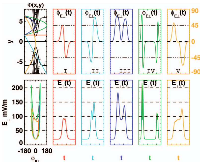
FIG. 3. (Color). Simulation of data acquisition across a planar, modeled curl-free electric field pattern for perpendicular \mathbf{E}_{\perp} in EFE. This model has been introduced to discuss the morphology of the largest (perpendicular to B ) components in the EFE. In no way does the model or its use imply or require that E_{\parallel} \equiv 0 . Upper left-hand panel illustrates the modeled equipotentials and depicts various colored worldlines of hypothetical spacecraft crossings of the EFE. Successive columns of panels illustrate the time profiles of E_{\perp}(t) and \phi_{E_{\perp}}(t) , using colors to match those that label the worldlines in upper left-hand panel. Lower left-hand panel depicts the phase portrait of all observers along the indicated worldlines in upper left-hand panel. The union of all points in the upper left-hand panel would “paint” the interior of the phase portrait that is presently delineated in lower left hand panel. Such arguments show that the data in individual columns in Fig. 2 may be modeled in this way, but that the entire burst cannot be represented by just one such structure as in the upper left hand corner.
